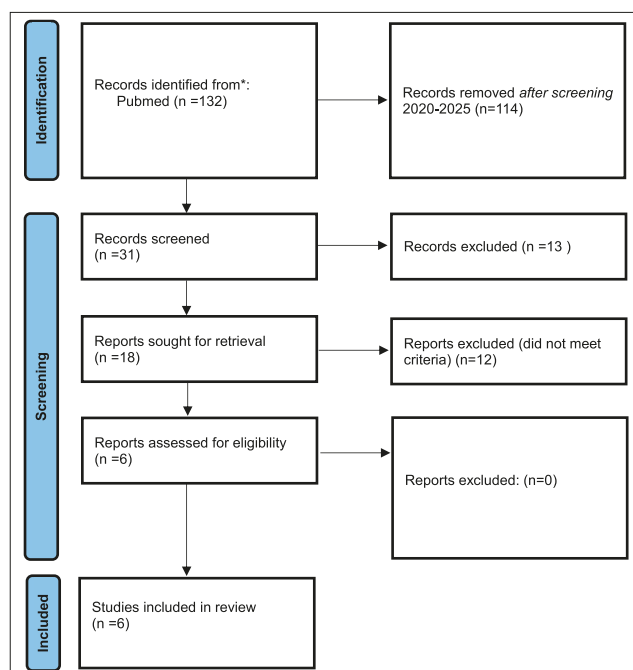
Figure 1. Prisma diagram
